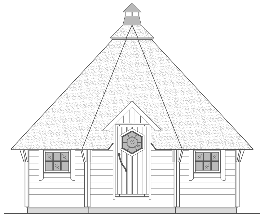
ARCTIC FINLAND HOUSE GRILLKOTA 17 m 2
